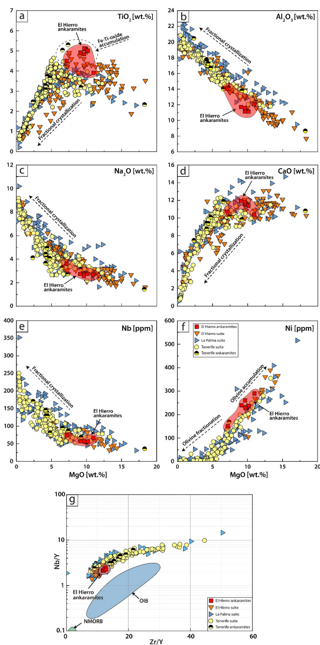
Figure 4. (a–f) MgO variation diagrams for El Hierro post-collapse ankaramites as well as other representative volcanic rocks from El Hierro, La Palma, and Tenerife. The overall curved major and trace element trends indicate fractional crystallization as the dominant process controlling compositional variations for El Hierro, La Palma, and Tenerife volcanic rocks, while trace element data also indicate a degree of accumulation. Additional data from Abratis et al. (2002); Carracedo et al. (2001); Deegan et al. (2012); Klügel et al. (2011); Pellicer (1979); Schmincke (1982). (g) Nb/Y versus Zr/Y plot for El Hierro post-collapse ankaramites and other El Hierro, La Palma, and Tenerife volcanic rocks with reference fields for normal mid-ocean ridge basalt (NMORB) and OIB (after Fitton et al., 1997, 2003). El Hierro ankaramites and most other Canary Island volcanic rocks plot outside the reference field for NMORB and OIB because they are results of fractionation and accumulation rather than being primary melts. Additional data from Abratis et al. (2002); Carracedo et al. (2001); Deegan et al. (2012); Klügel et al. (2011); Schmincke (1982).
