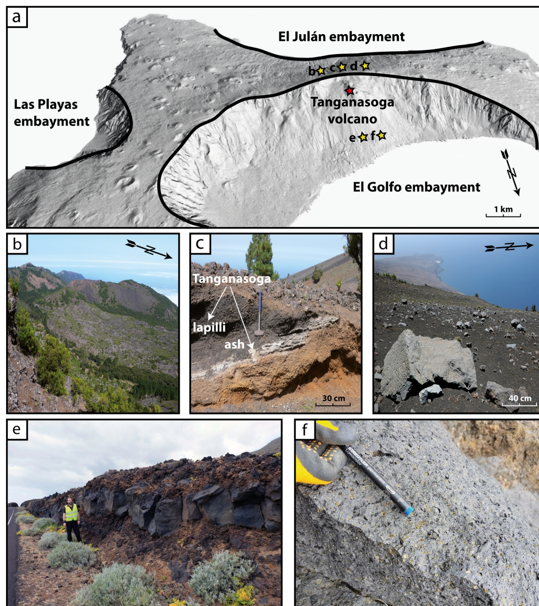
Figure 2. (a) Oblique view of the El Golfo collapse embayment (Source: GRAFCAN (2024)). Photo locations of panels (b) to (f) are indicated by yellow stars, the Tanganasoga volcano is indicated by a red star. (b) Summit vent of Tanganasoga and post-collapse ankaramite lava flows viewed from the rift zone crest above the volcano. (c) Layers of pyroclastic material on the rift above the Tanganasoga edifice. (d) Ankaramite blocks and ash deposits erupted from Tanganasoga volcano that were deposited on the crest of the rift zone. (e and f) Example of an ankaramite lava flow on the northwestern flank of the Tanganasoga edifice with exceptionally high contents of large clinopyroxene and olivine crystals.
