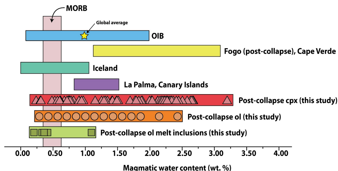
Figure 6. Comparison of magmatic water contents of El Hierro post El Golfo collapse eruptives, post-collapse Fogo eruptives (Cape Verde), La Palma (Canary Islands), Iceland, and other Ocean Island Basalt (OIB) and Mid-Ocean Ridge Basalt (MORB) compositions. Standard MORB (UOB reference material) values are from Bindeman et al. (2022); water values for OIBs are from Deegan et al. (2012); Dixon et al. (1997); Dixon and Clague (2001); Gurenko and Schmincke (2000); Kovalenko et al. (2007); Moore (1970); Sides et al. (2014); Wallace (1998a, 1998b); Weis et al. (2015). Values for Fogo are from DeVitre et al. (2023) and Lo Forte et al. (2023), for La Palma from Weis et al. (2015), and Iceland from Radu et al. (2023).
