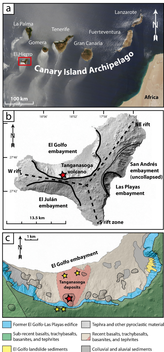
Figure 1. (a) Satellite map showing the location of El Hierro in the Canary archipelago (red box; Carracedo & Troll, 2016). (b) Overview DEM map of El Hierro showing the three main rift zones of the island (stippled lines) and the main landslide embayments (solid lines) DEM source: GRAFCAN (2024). The Tanganasoga volcano is a prominent feature located inside the El Golfo landslide embayment and is marked with a red star. (c) Simplified geological map of the El Golfo collapse embayment showing the distribution of different volcanic rocks and pyroclastic material. Ankaramite samples were collected from pyroclastic deposits on the rift zone above the El Golfo embayment and from lava directly within the embayment. Sampling locations are marked with yellow stars (DEM source: GRAFCAN (2024)).
